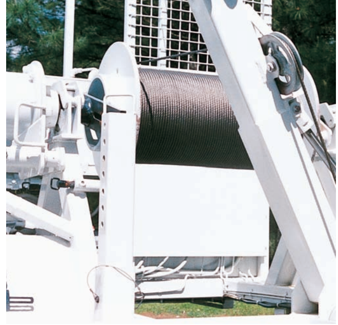
UNDERGROUND PULLER
